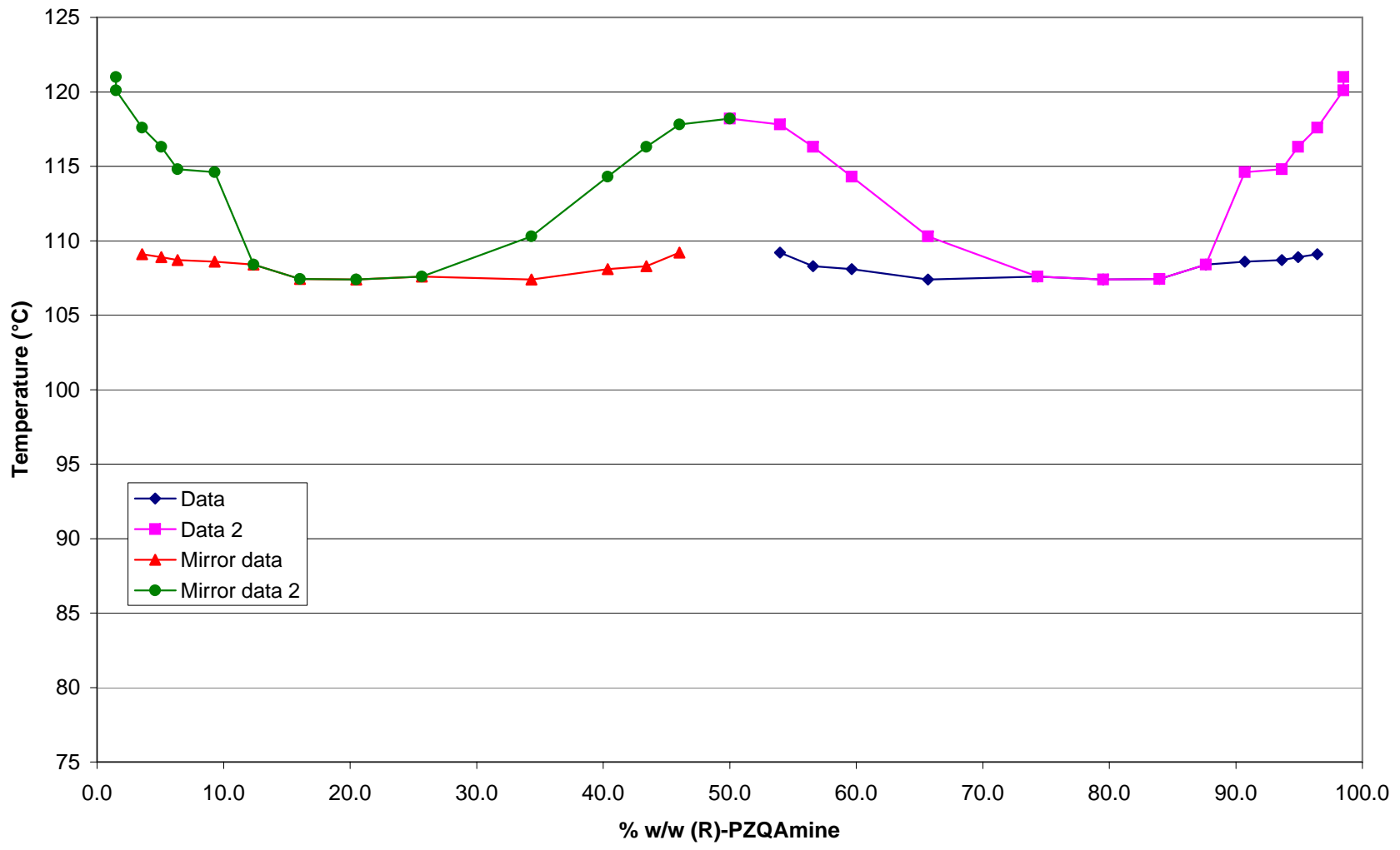
Phase Diagram for PZQAmine via Onset of Melting by DSC Data collected at Almac Sciences in Oct 2011
